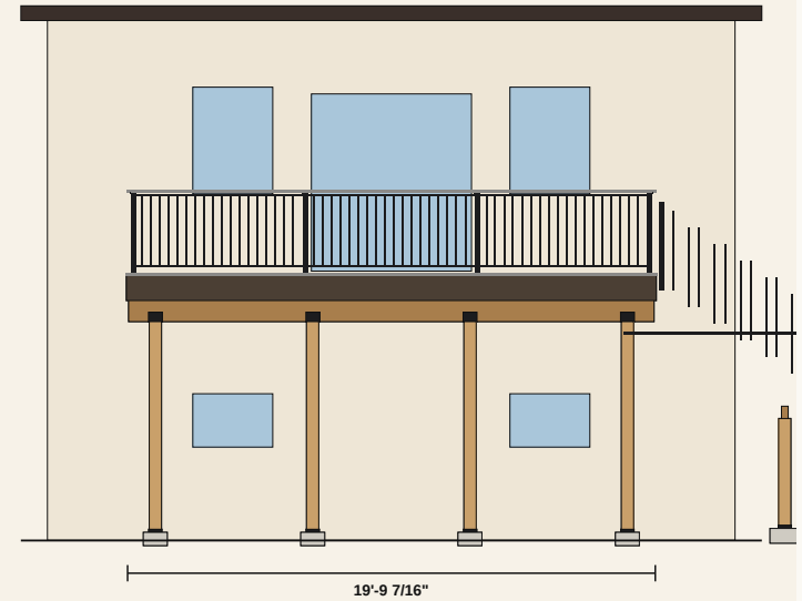
FRONT ELEVATION — from the yard
